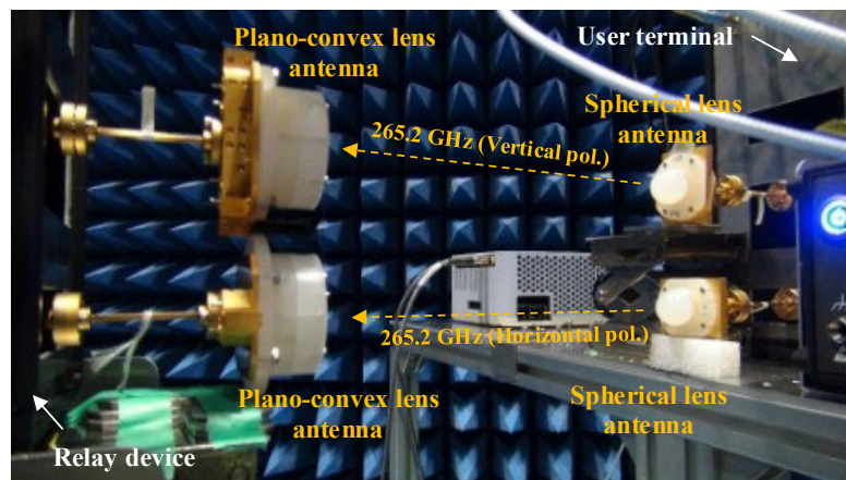
(b) Photograph zoomed up terahertz-band part.
