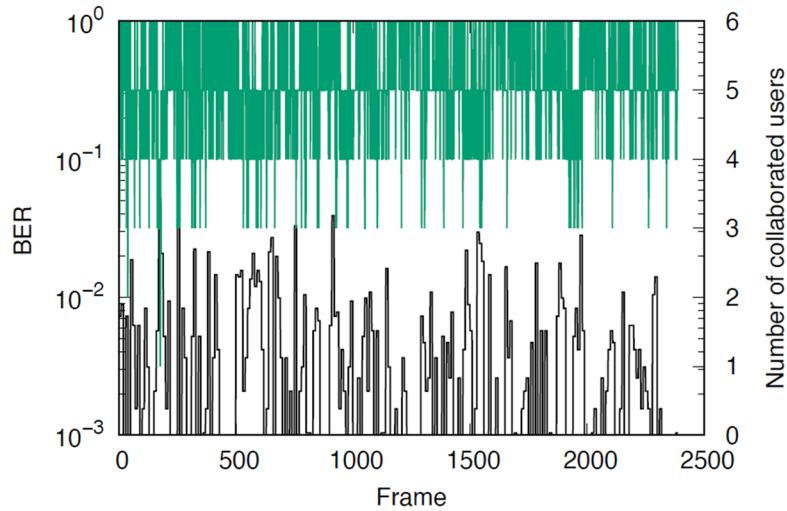
Fig. II-3-6 BER averaged over 10 packets and number of collaborated
