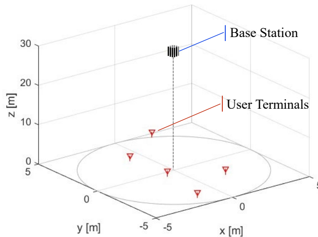
Figure II-1.8-4. Simulation environment.
