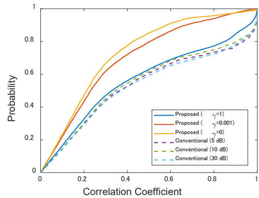
Fig. II-1.7-4. CDF of channel correlation.
