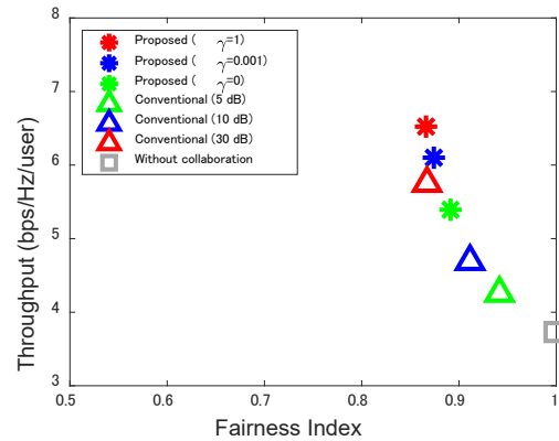
Fig. II-1.7-5. Throughput vs. fairness.
