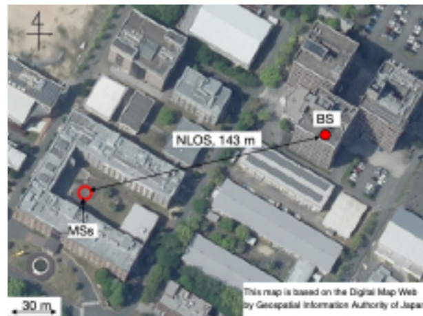
Fig. II-3-2 Measurement campaign field and layout.
