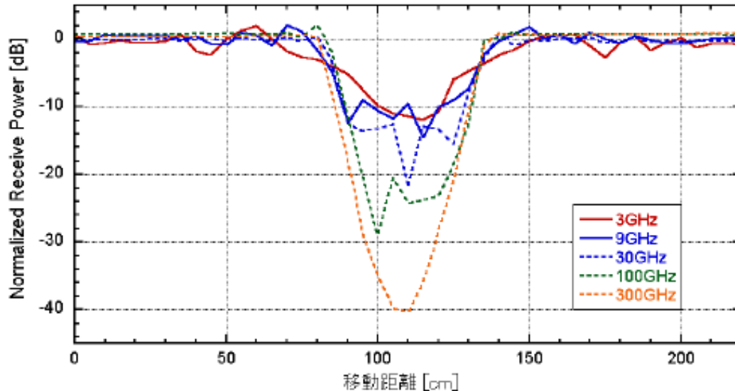
Fig. 3-2 Example of shielding loss measurement results [1]
