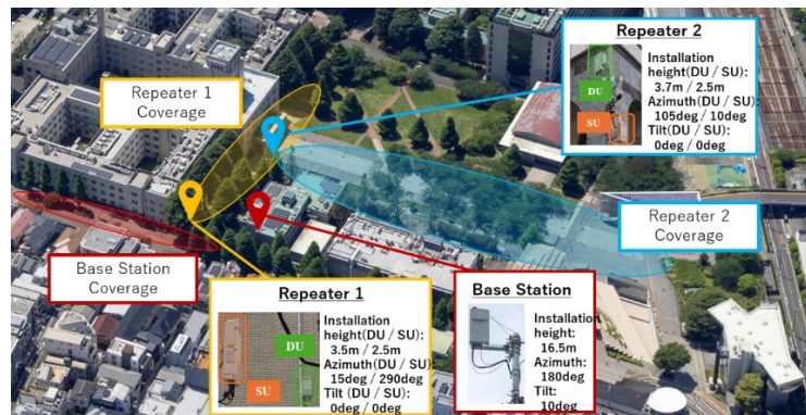
Fig. 5-14 Millimeter Wave Base Station Coverage and Repeater Deployment at Ookayama Campus
