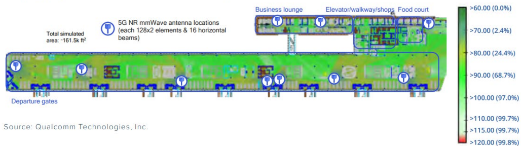
Fig. 5-5 Installation example of 5G millimeter wave base stations at airports and its measurement result [1]
