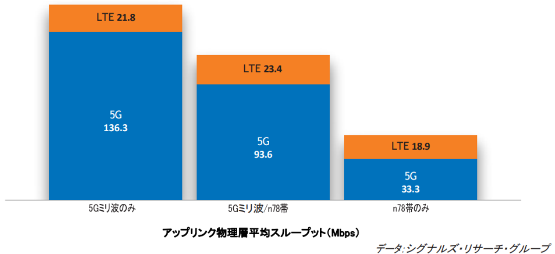
Fig. 5-7 5G millimeter wave uplink throughput mobile measurement outdoors [2]-[3] (English version is available in [3] with registration)
