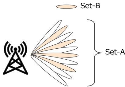
Fig. 4-16 Example of Beam Set A and Beam Set B (Determining the optimal beam from Beam Set A based on the measurement of Beam Set B using AI/ML)
