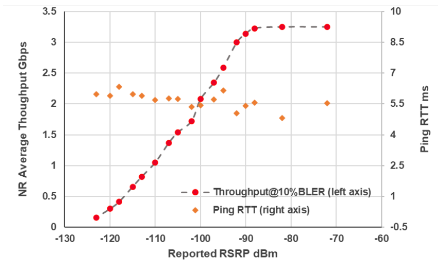
Fig. 5-3 5G millimeter wave throughput and round-trip delay
