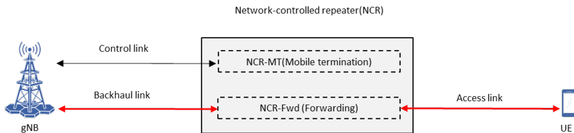
Fig. 4-4 Network controlled repeaters [13]
