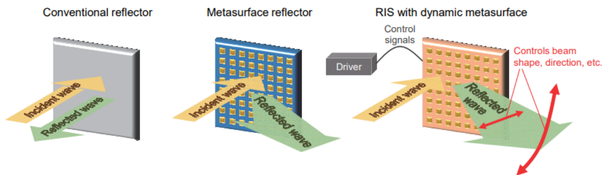
Fig. 4-7 Conceptual diagram of RIS using metasurface technology
