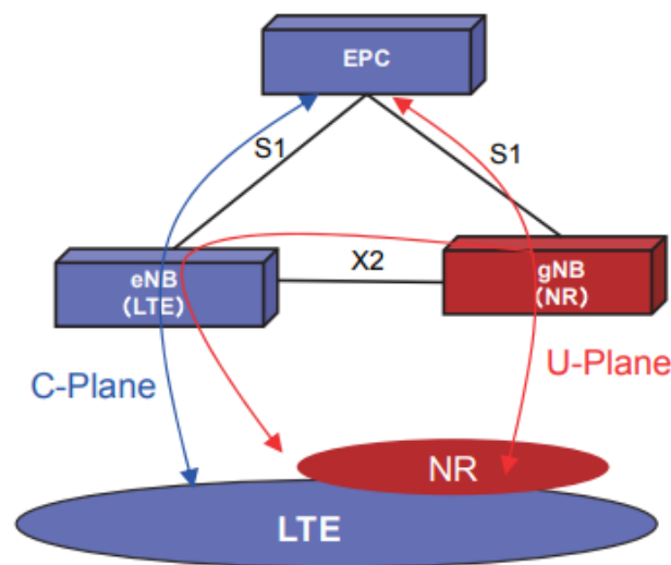
Fig. 4-11 Concept of LTE-NR dual connectivity
