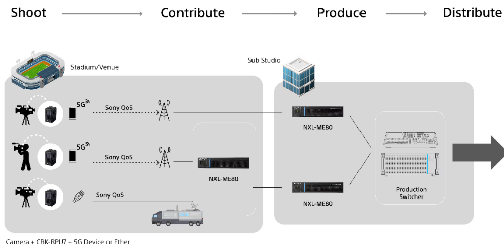
Fig. 8-9 Sony's Video Transmission Solution
