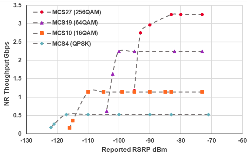
Fig. 5-2 5G millimeter wave throughput
