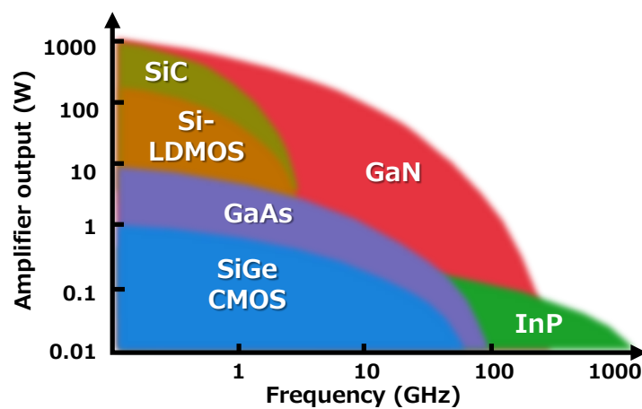
Fig. 4-8 Relationship between frequency and amplifier output
