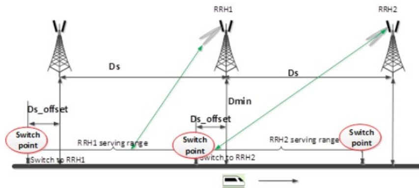
(a) Uni-directional deployment
