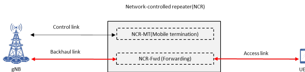
Fig. 4-4 Network controlled repeaters [13]
