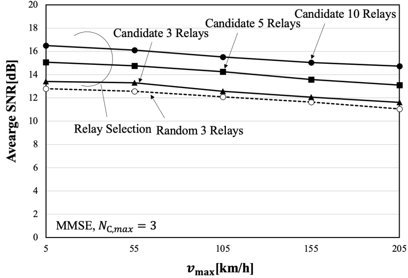
Figure II-1.2-2 theoretical relay selection in the proposed relaying
