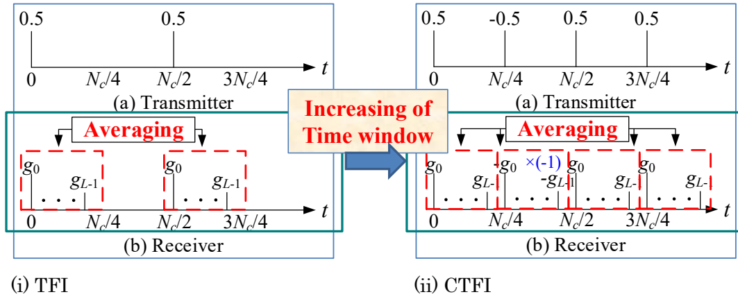
Fig. II-1.4-2. Time window averaging by TFI and CTFI.
