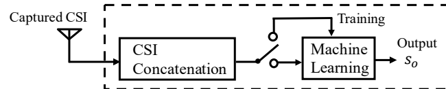
Figure III-7.2 Block diagram of the CSI acquisition terminal.
