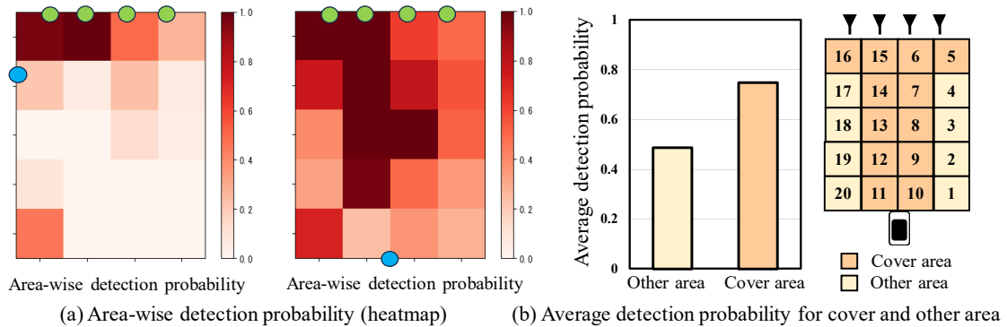
Figure III-7.5 Average detection probability for large-scale indoor experiment scenario [9].
