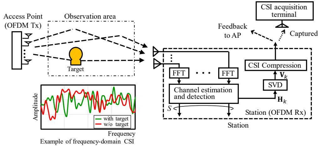
Figure III-7.1 Principles of CSI acquisition for WLAN-based device-free localization.
