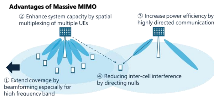
Fig.1-1 Advantages of Massive MIMO
