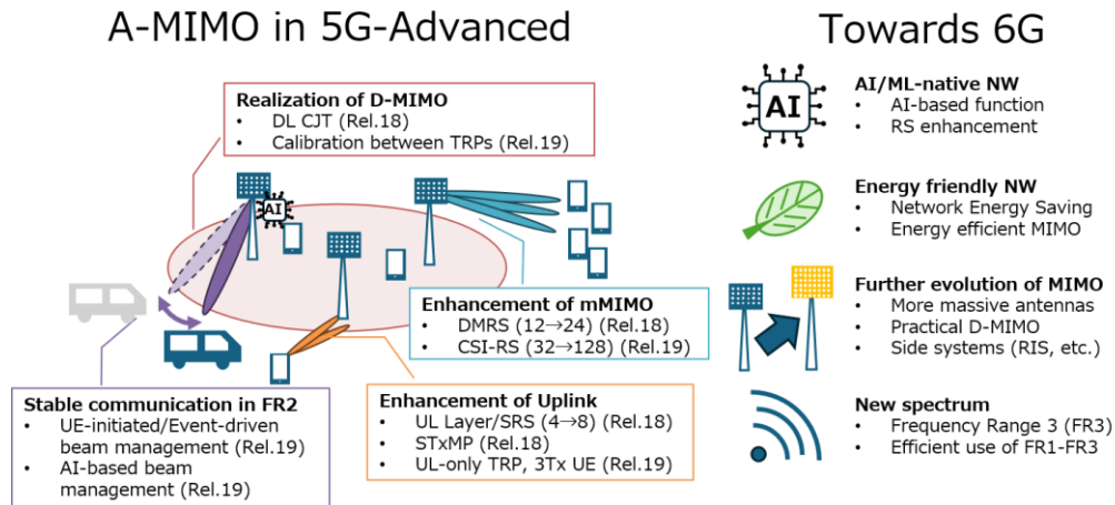
Fig. 3-1 Recent activities related Advanced MIMO in 3GPP
