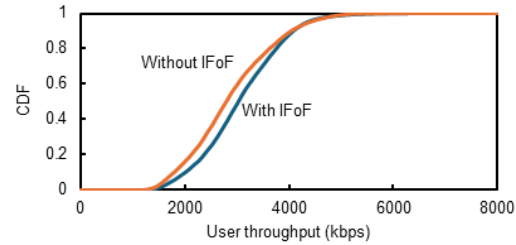
Fig. 1-7 Throughput with/without IFoF.
