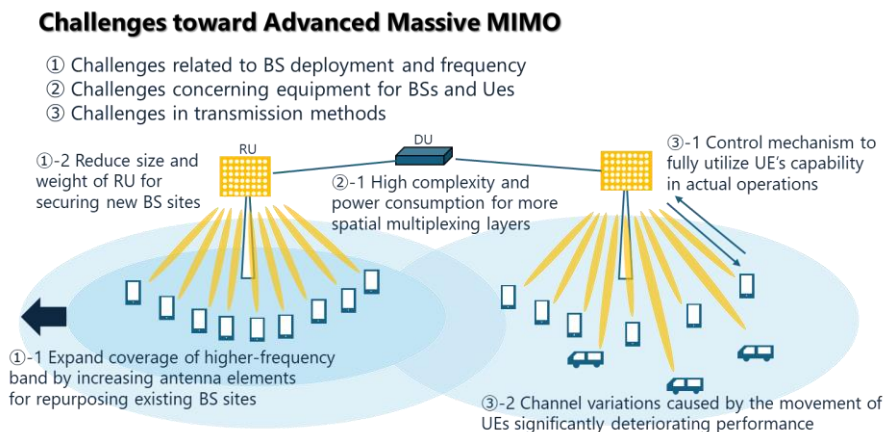
Fig.1-2 Challenges toward Advanced Massive MIMO
